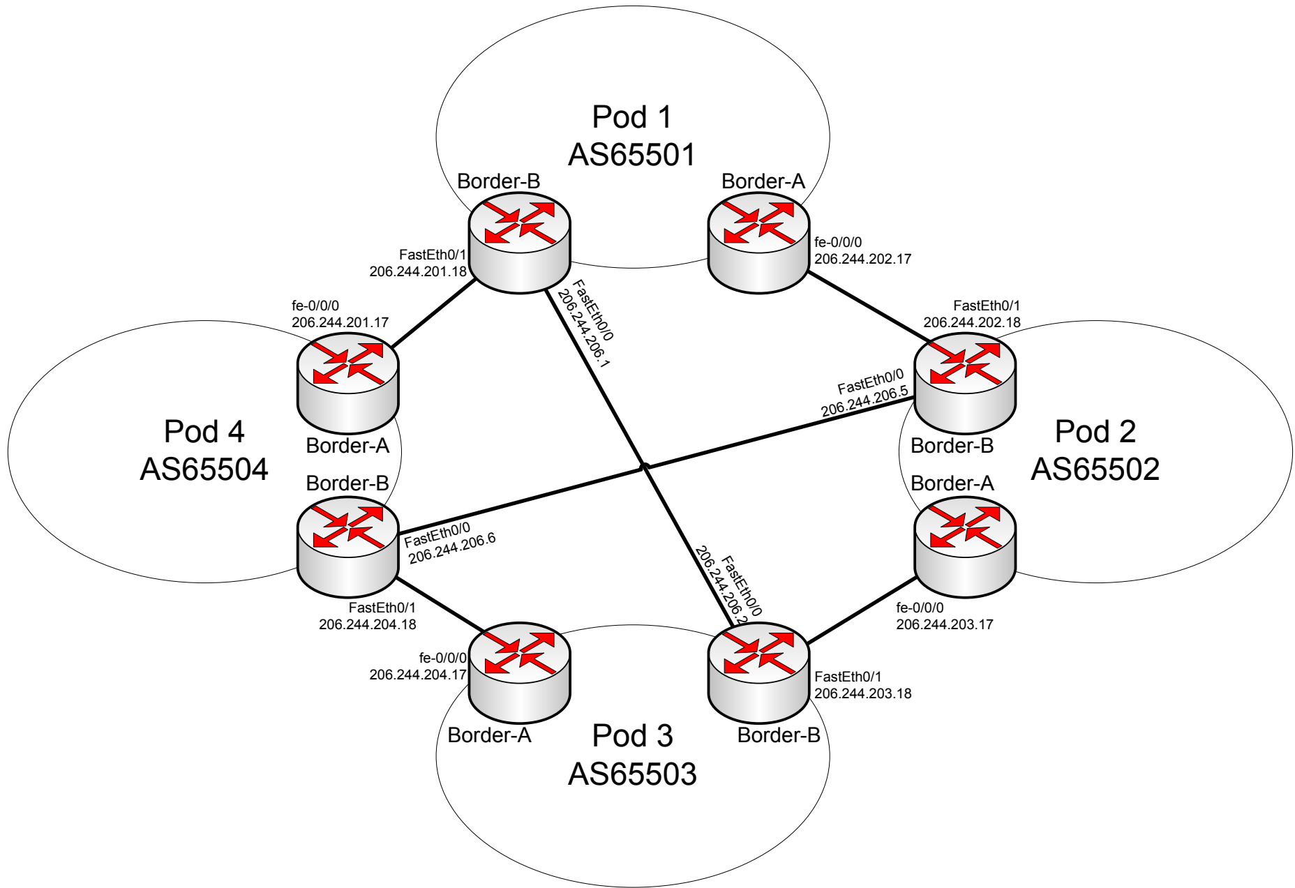
Inter-Pod Diagram IPv6 Unicast Workshop
